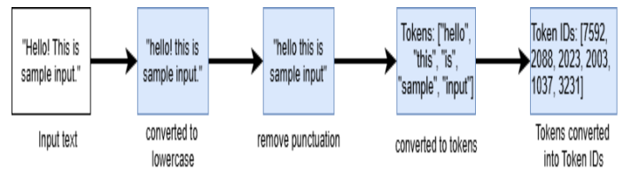
Figure 2: Conversion of text inputs into token-IDs
